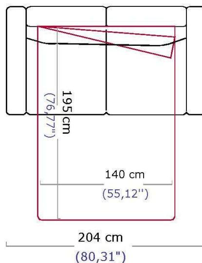
320 CANAPÉ 3 PLACES – Couchage 140x195 cm 3-SEAT SOFA – 140x195 cm sleeping area SOFÁ 3 PLAZAS – Colchón 140x195 cm
