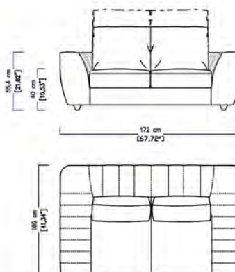
IM04 CANAPE 2 PLACES IM04 2-SEATER SOFA IM04 SOFA 2 PLAZAS
