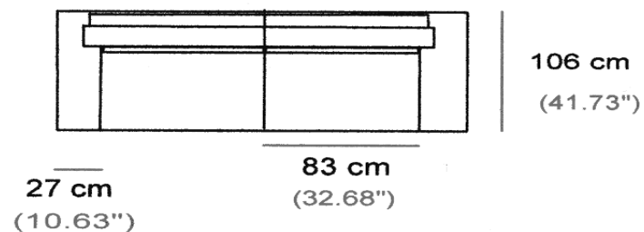
CANAPE 3 PLACES 3-SEAT SOFA SOFA 3 PLAZAS
