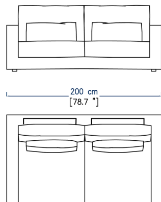
LB02 CANAPE 2 PLACES 1/2 2.5-SEATS SOFA SOFÁ 2 PLAZAS 1/2
